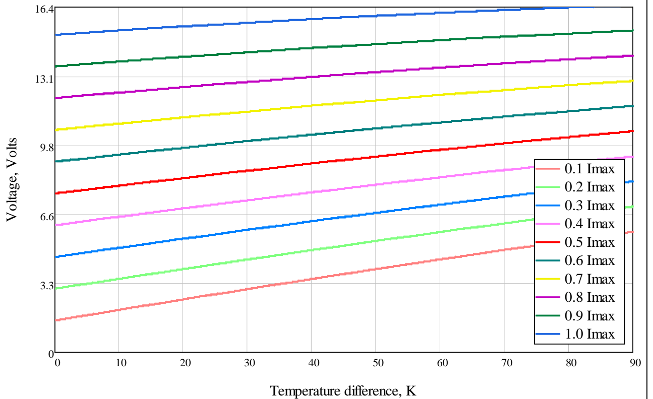
The Voltage vs. Temperature Difference at T_h=50^\circ\text{C} for Different I_{max}
