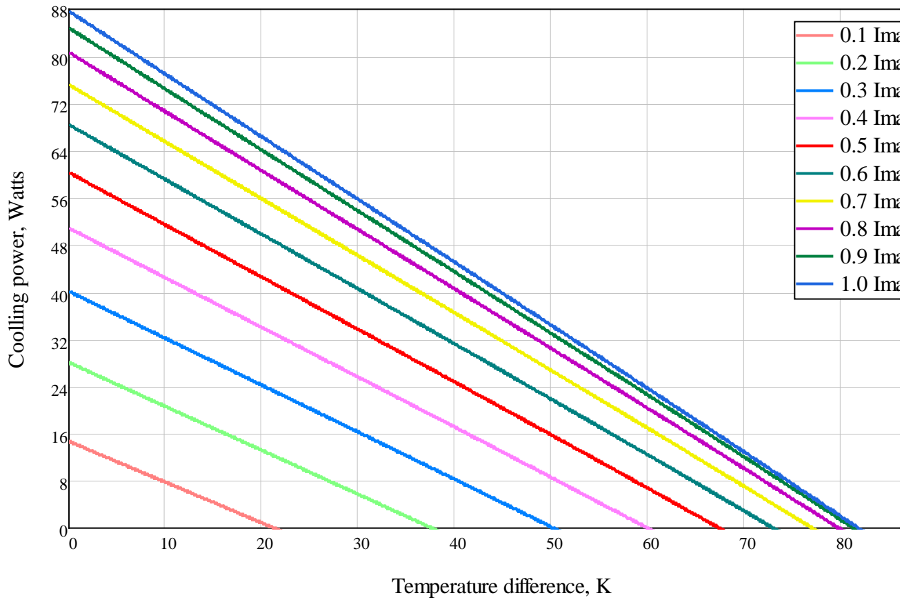
Cooling Power vs. Temperature Difference at T_h=50^\circ\text{C} for Different I_{max}
