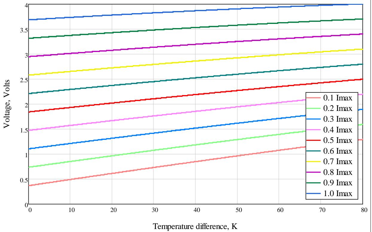
The Voltage vs. Temperature Difference at T_h=50^\circ\text{C} for Different I_{max}
