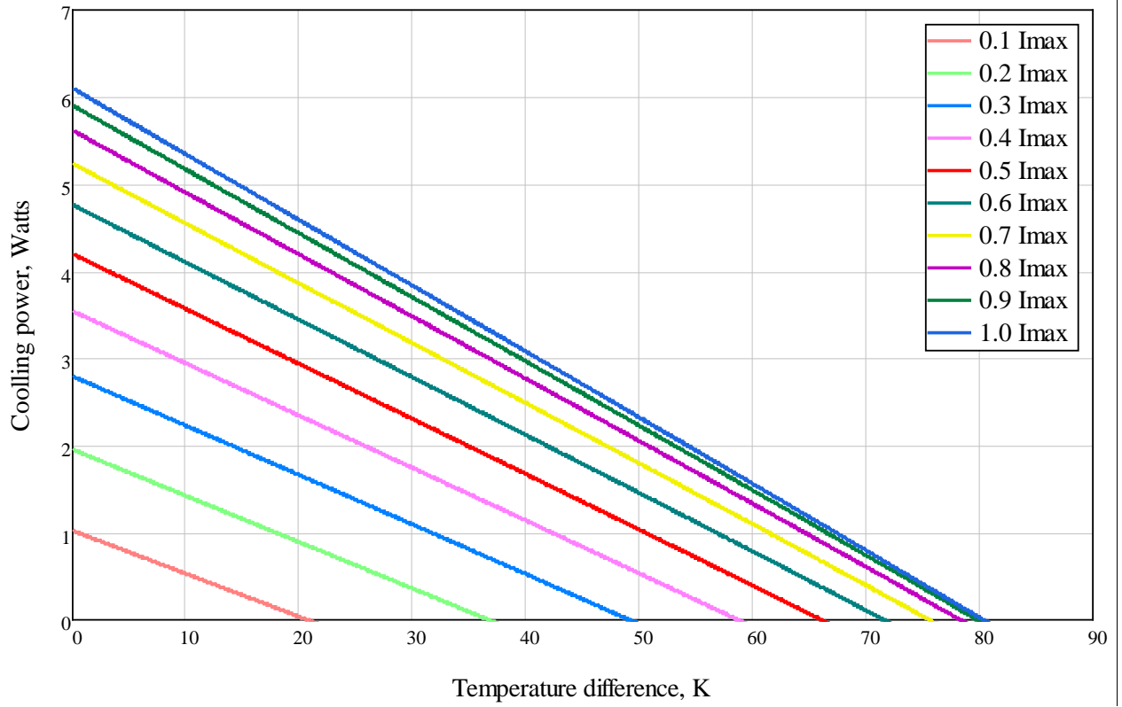
Cooling Power vs. Temperature Difference at T_h=50^\circ\text{C} for Different I_{max}
