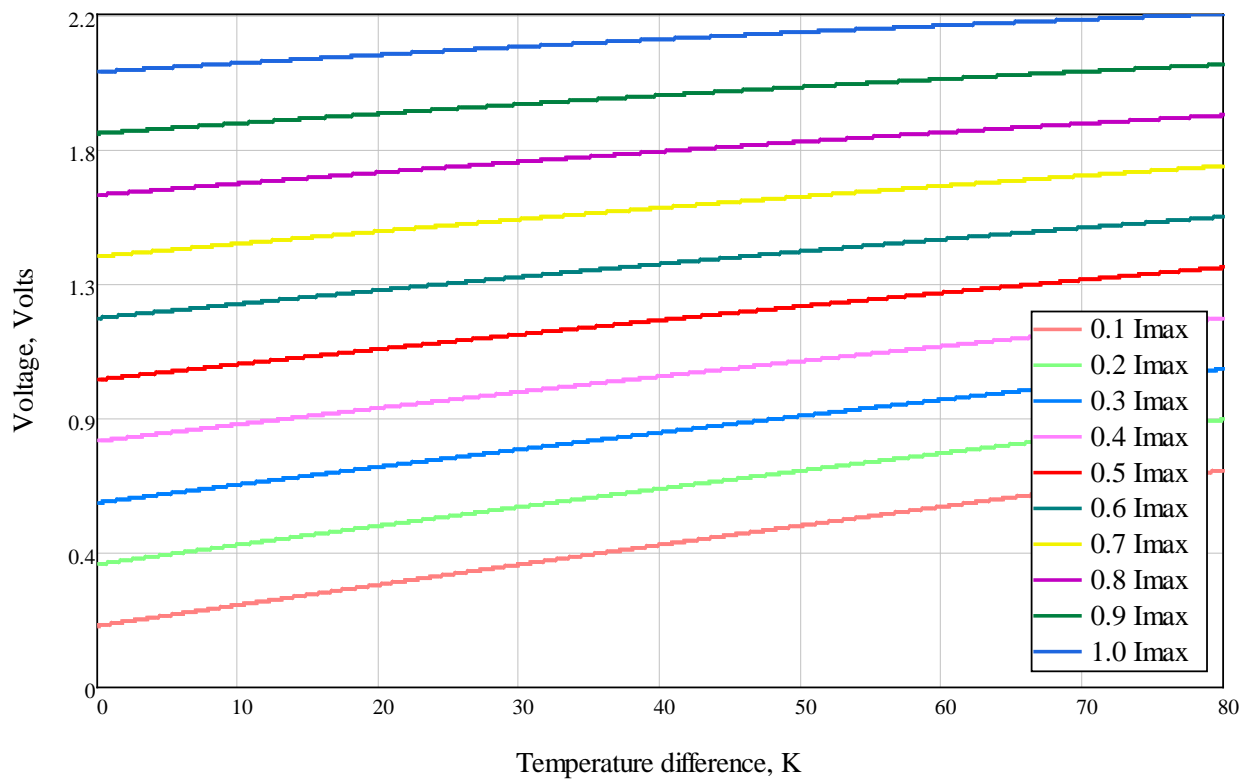
The Voltage vs. Temperature Difference at T_h=50^\circ\text{C} for Different I_{\text{max}}
