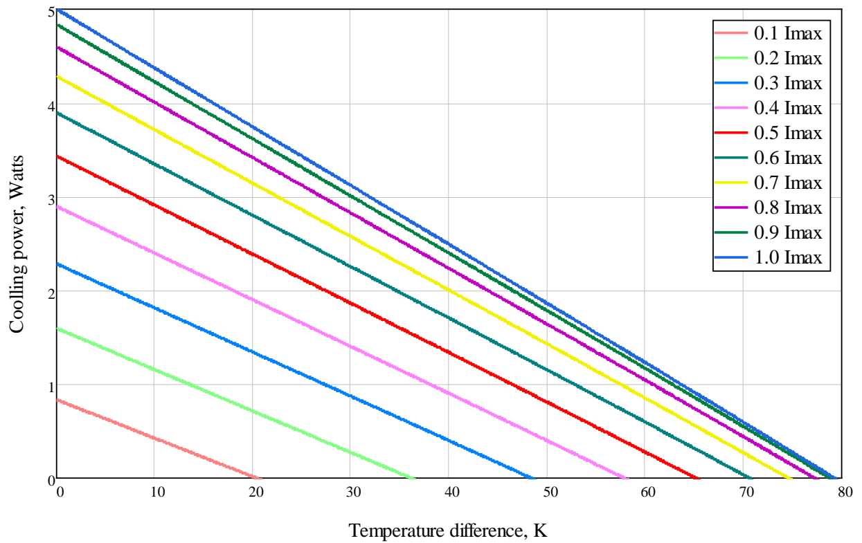
Cooling Power vs. Temperature Difference at T_h=50^\circ\text{C} for Different I_{\text{max}}
