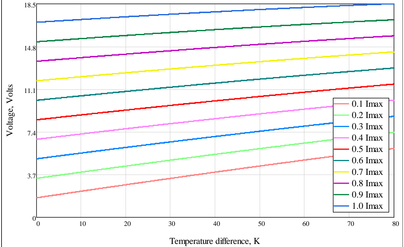
The Voltage vs. Temperature Difference at Th=50°C for Different I max
