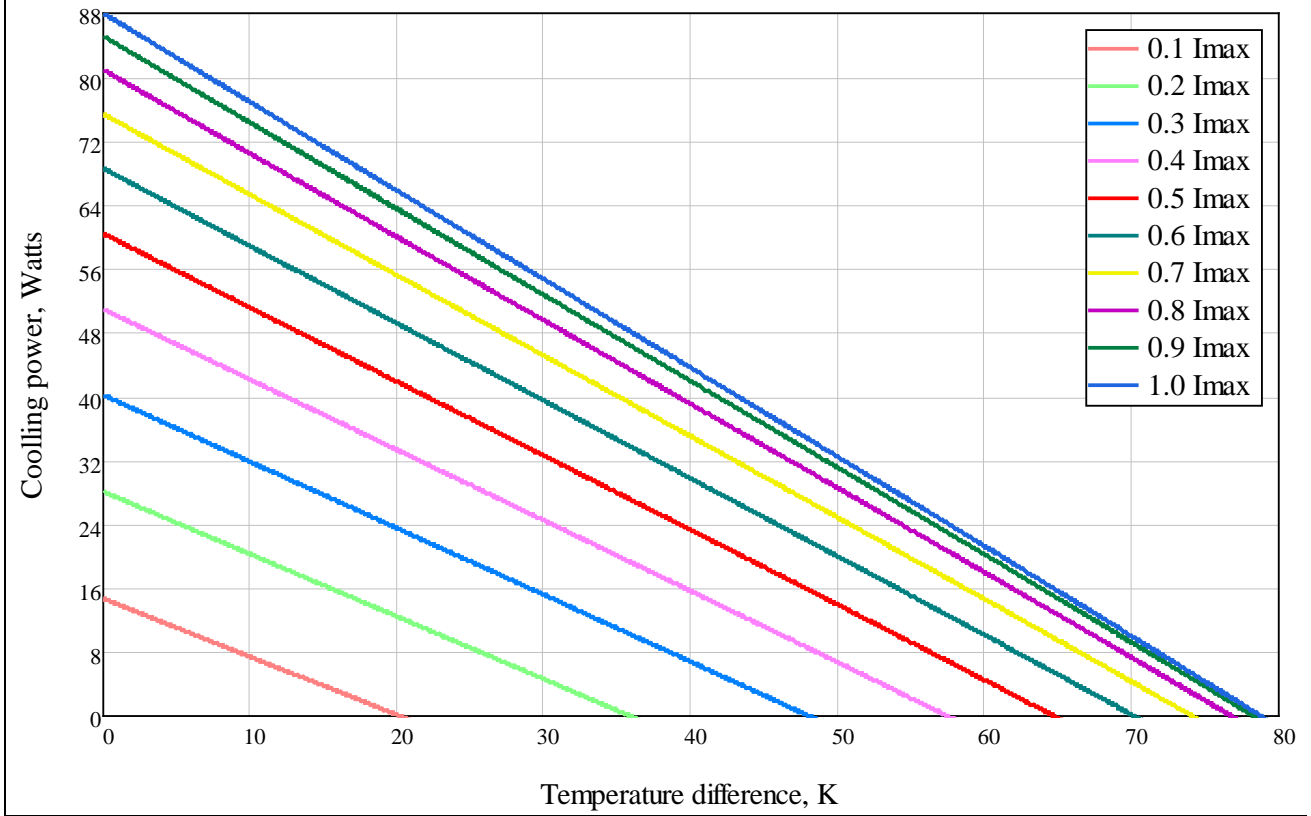
Cooling Power vs. Temperature Difference at Th=50°C for Different I max
