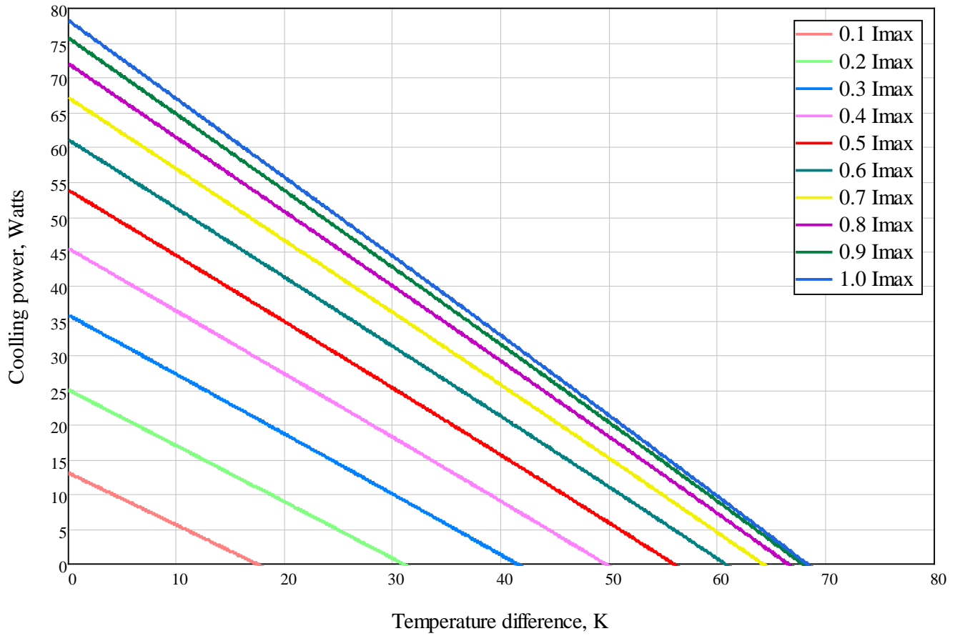
Cooling Power vs. Temperature Difference at T_h=27^\circ\text{C} for Different I_{\text{max}}
