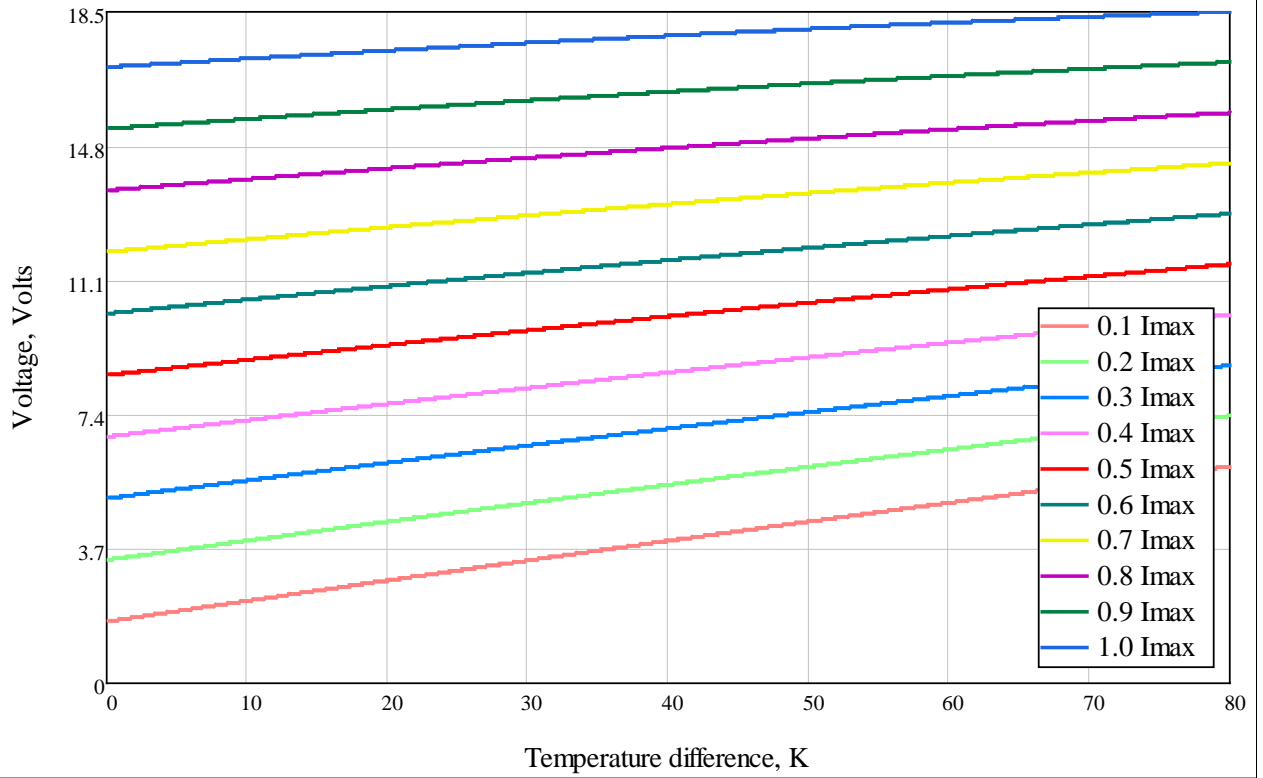
The Voltage vs. Temperature Difference at T_h=50^\circ\text{C} for Different I_{\text{max}}
