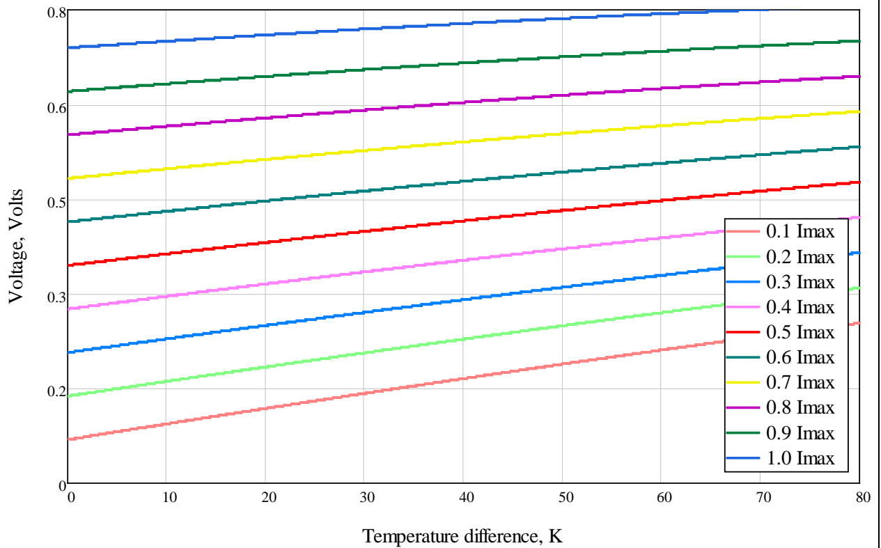
The Voltage vs. Temperature Difference at T_h=27^\circ\text{C} for Different I_{\text{max}}
