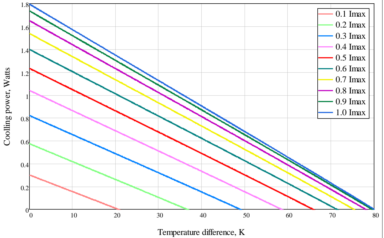
Cooling Power vs. Temperature Difference at T_h=50^\circ\text{C} for Different I_{max}
